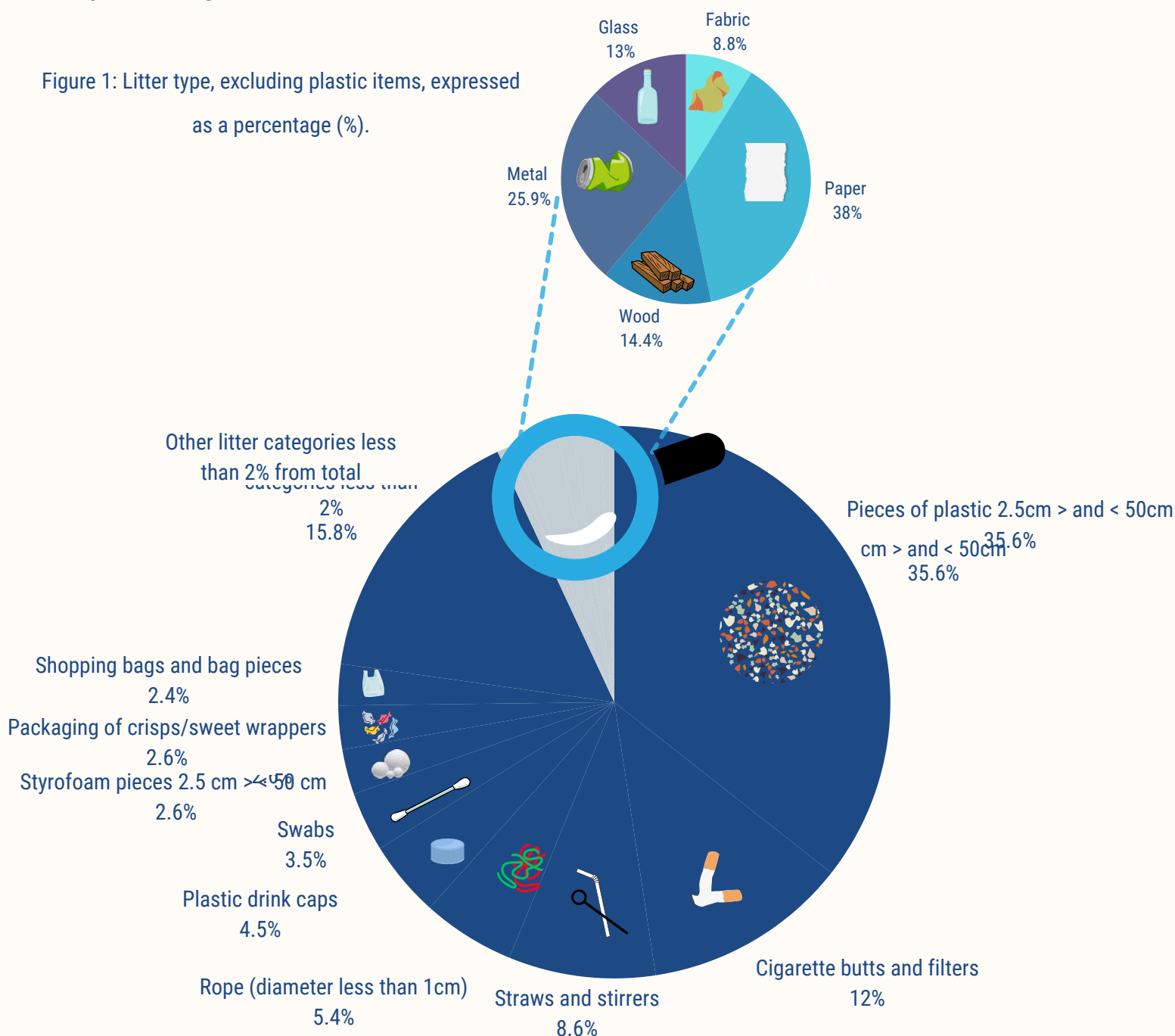
Figure 2: Litter type expressed as a percentage (%).
