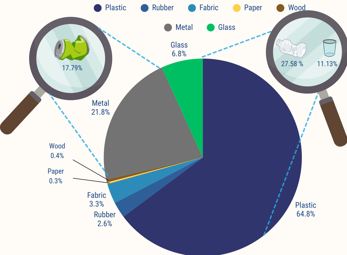
Figure 4: Collected types of benthic litter per underwater cleanup, expressed as a percentage of the total items (%).
