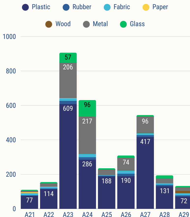
Figure 5: Collected and recorded benthic litter per category per activities
