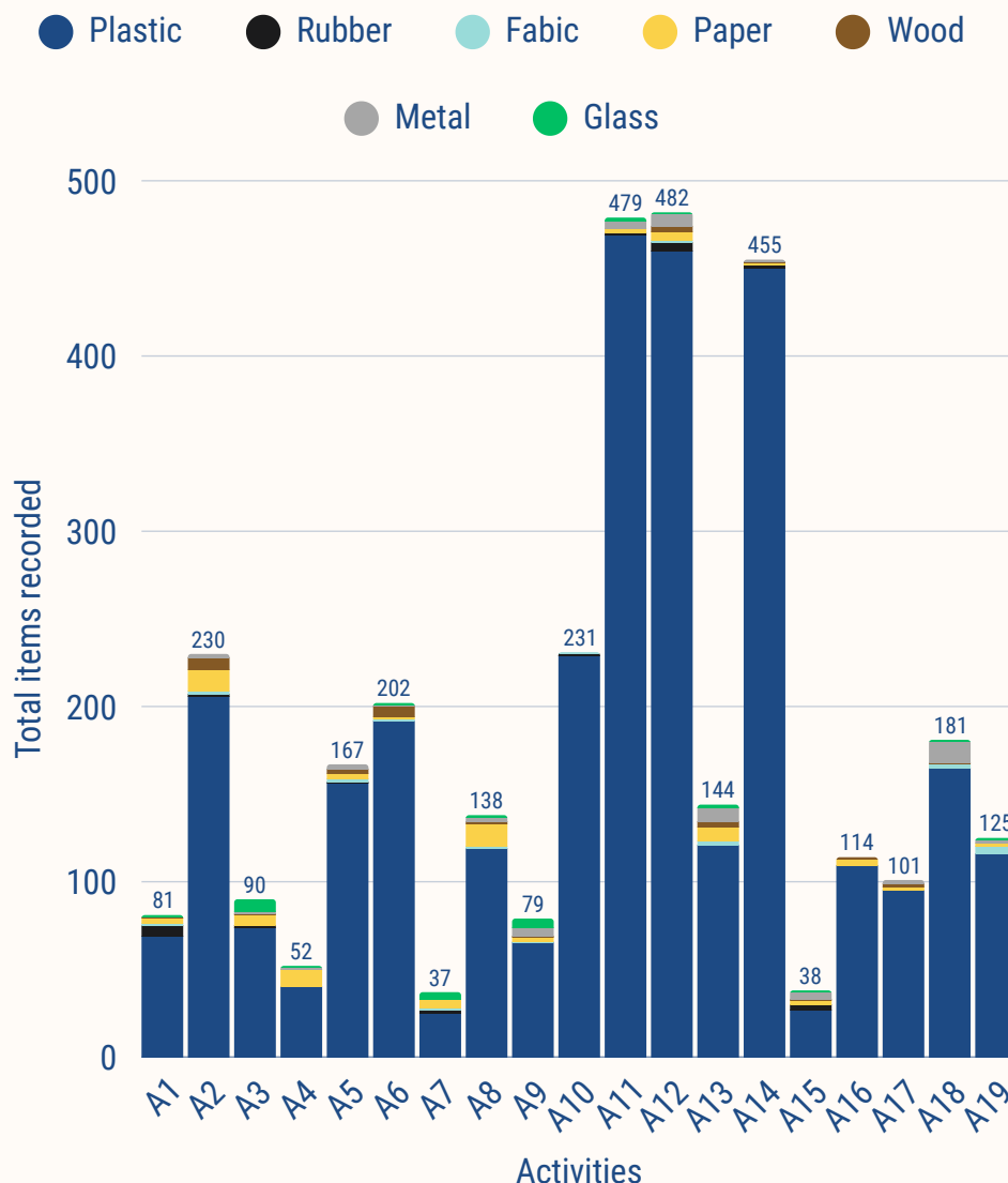
Figure 3: Recorded types of litter, per activity, expressed as percentage (%).
